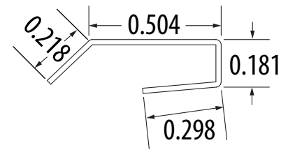
PN0484340 TFCG-5/16 (Channel w/ Guard for 5/16" Wiper)
