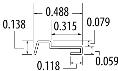
PN0484345 PR2 Channel Guard
