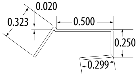
PN0484341 TFCG-1/2 (Channel w/ Guard for 1/2)
