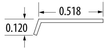
PN0484346 TFG-1/8 (Guard for 1/8" Wiper)
