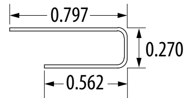
PN0484343 TFC-3/4 (Channel for Wiper TFW-3/4)
