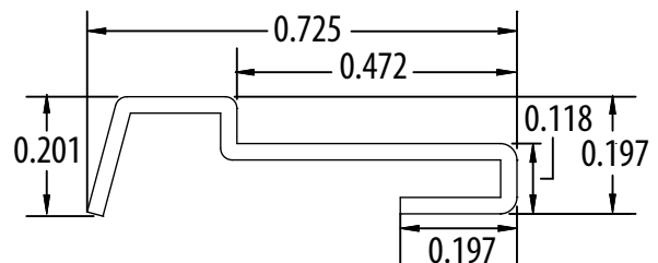
PN0484344 TFW-N4 (Channel w/ Guard)
