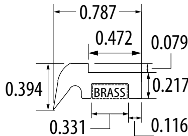
PN0484331 TSA-M19 Wiper (Brass bar recommended, sold separately)
