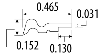
PN0484334 PR2 Wiper
