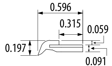
PN0484337 TFW-MA8/N6 Wiper
