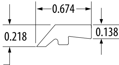
PN0484326 TFW-5/16N (5/16" Wiper w/ Ridge)
