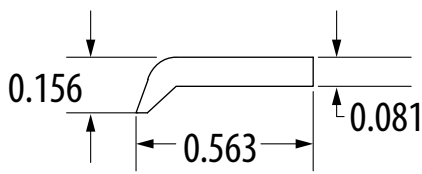
PN0484325 TFW-1/8 Wiper
