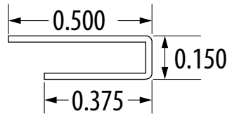
PN0484339 TFC-1/8 (Channel for TFW-1/8)
