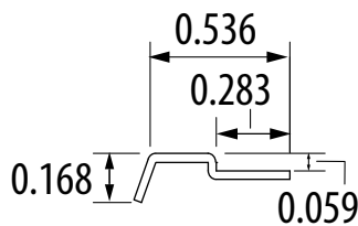
PN0484348 TFG-MA8/N6 (Guard for N6 Wiper)
