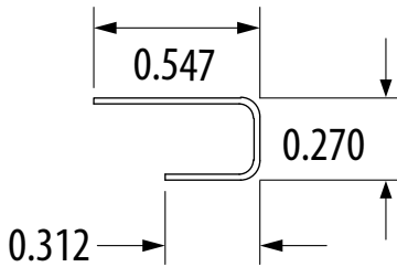
PN0484342 TFC-1/2 (Channel for Wiper TFW-1/2)
