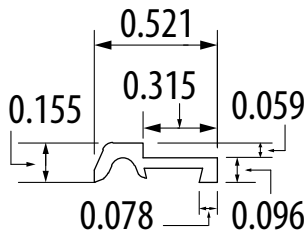
PN0484350 TFCG-741 (Channel & Guard for TFW-740 Wiper)
