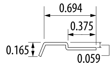
PN0484349 TFG-MA12/N7 (Guard for N7 Wiper)
