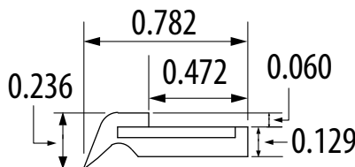
PN0484338 TFW-MA12/N7 Wiper
