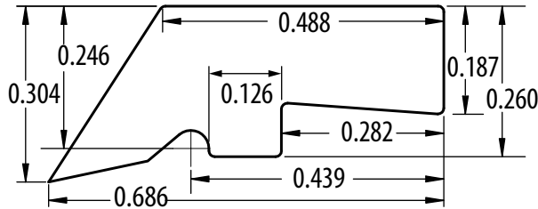
PN0484327 TFW-1/2N (1/2" Wiper w/ Ridge)
