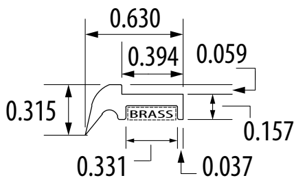
PN0484330 TSA-M16 Wiper (Brass bar recommended, sold separately)
