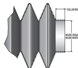
COLLAR
