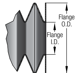
STANDARD FLANGE
